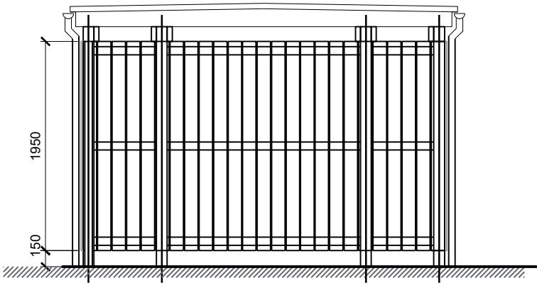
Rear Elevation
