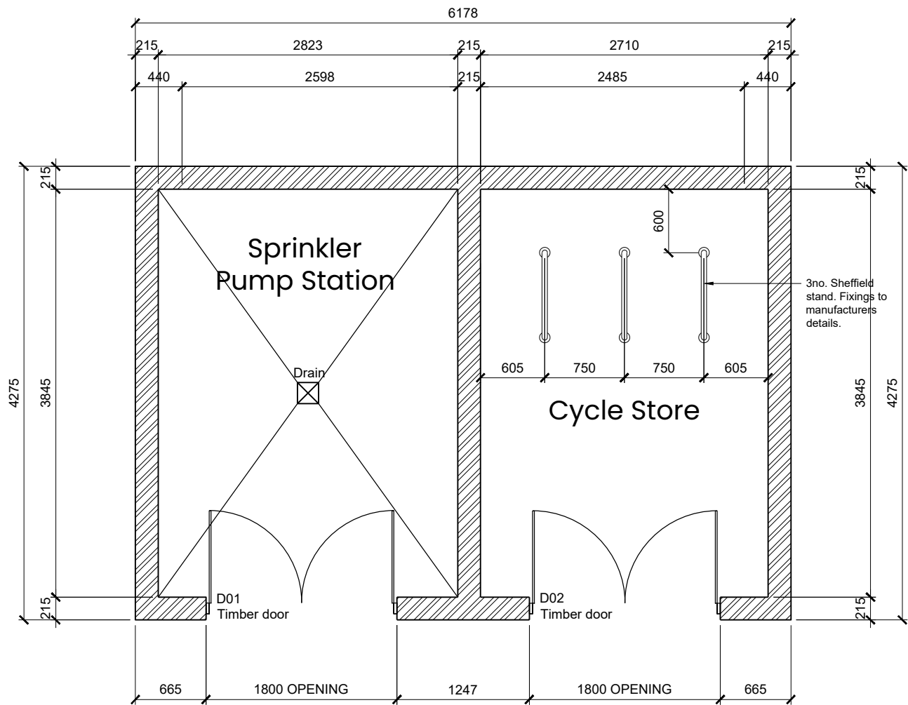
Floor Plan ■ Sprinkler Pump & Bike Store
