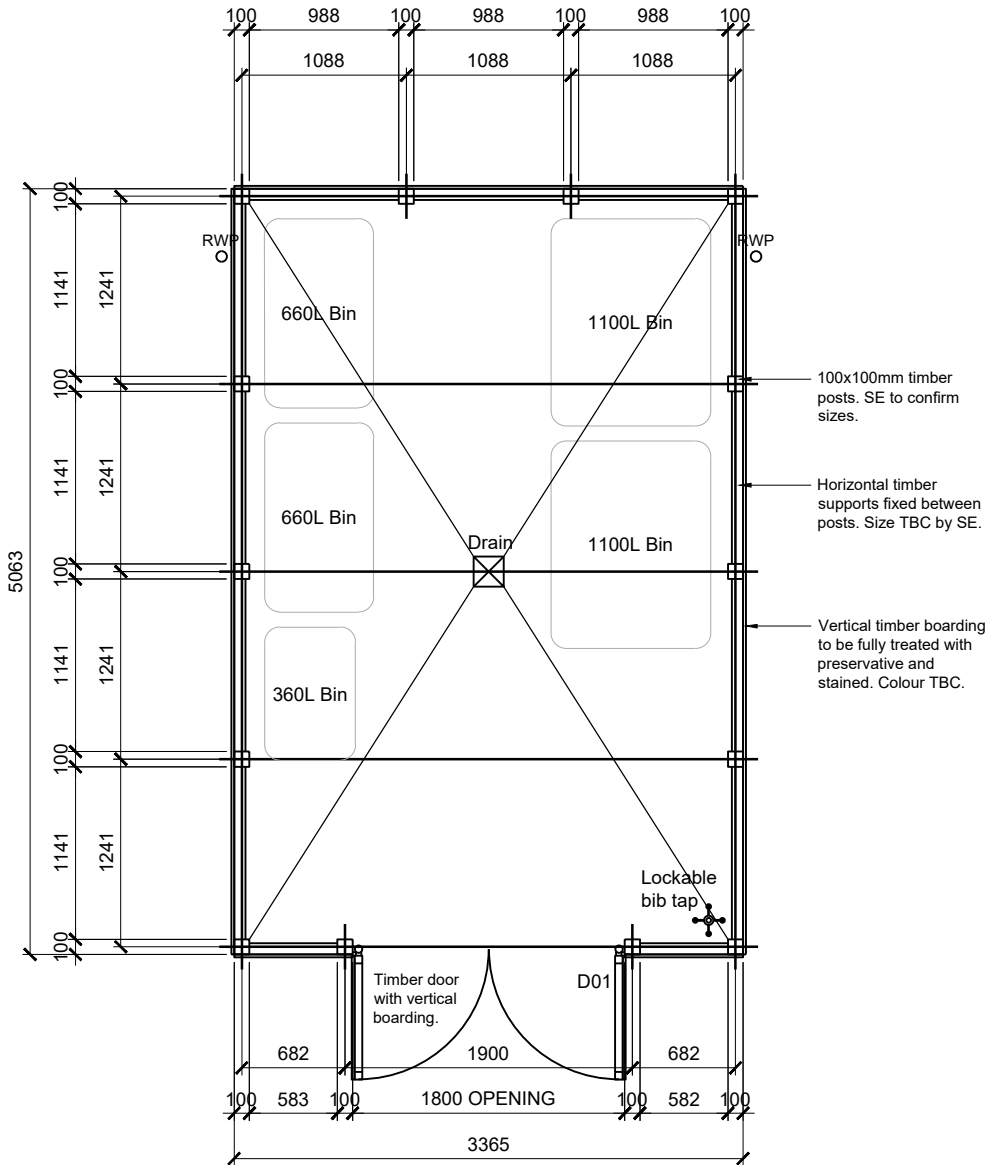
Floor Plan Bin Store C
