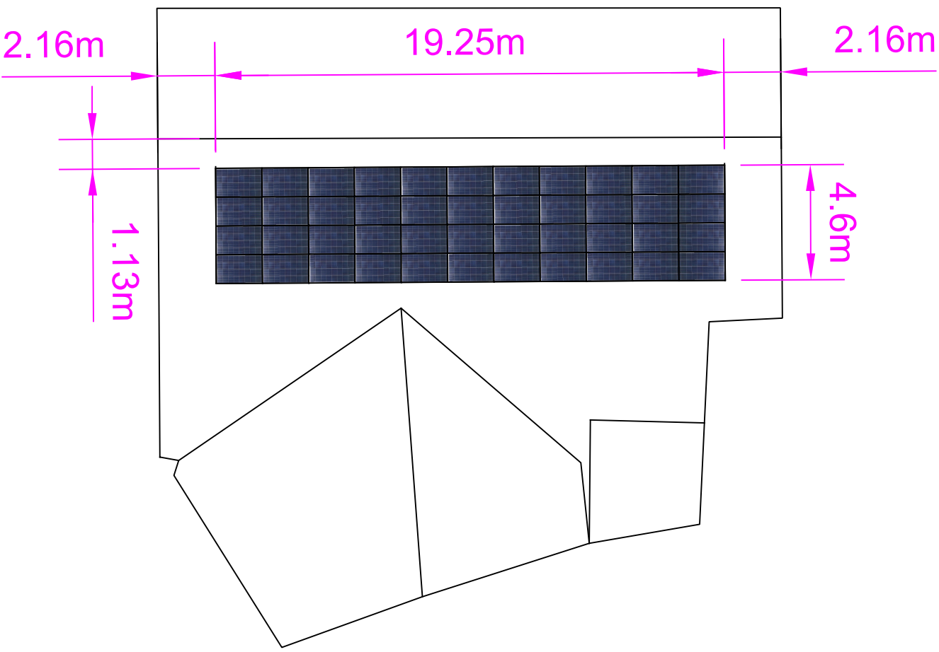
Proposed Roof Layout
