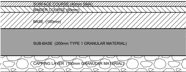
(2) 3 BITUMINOUS LAYER ACCESS ROAD AND HGV LOCATIONS
