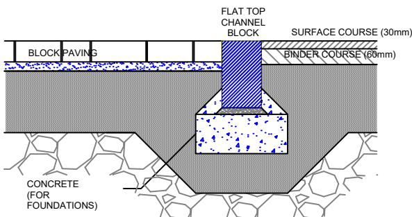
(1) 125MM WIDE FLAT TOP CHANNEL BLOCK ON 2 BITUMINOUS LAYER AND LIGHT VEHICLE LOCATIONS
