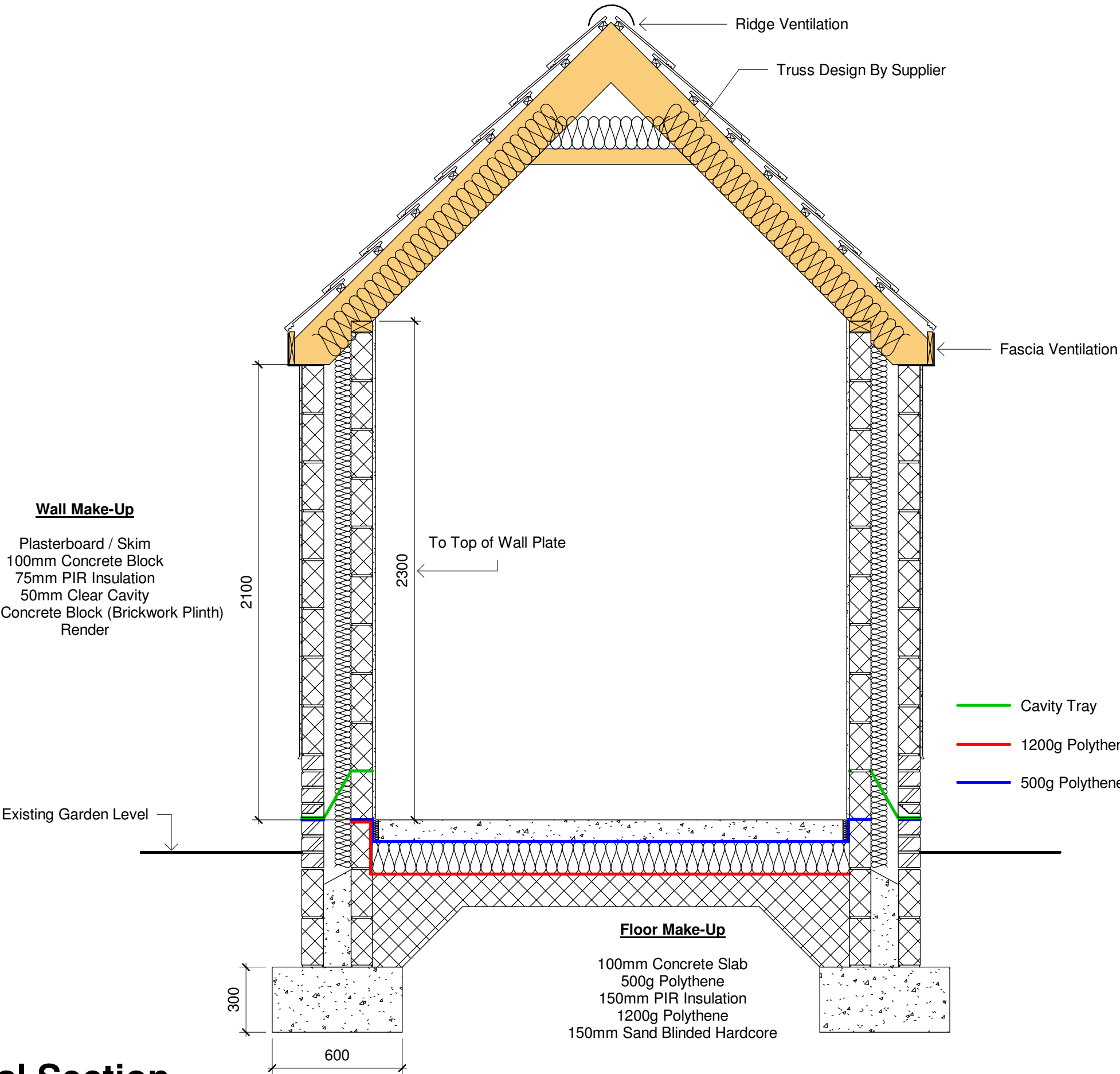
1 Typical Section 1 : 20
