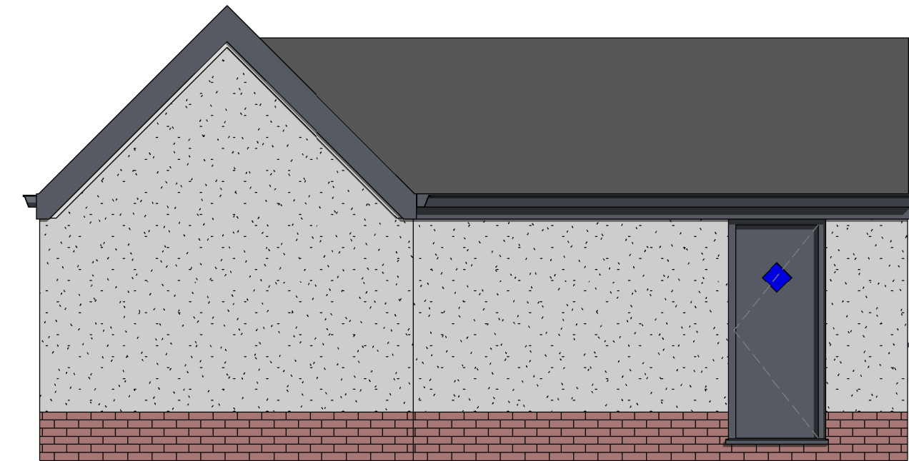
4 Left Elevation 1 : 50
