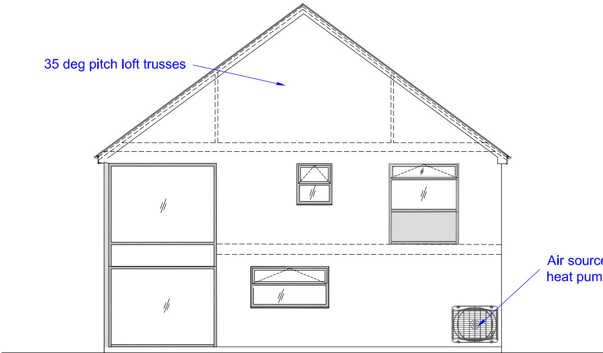
WEST ELEVATION
