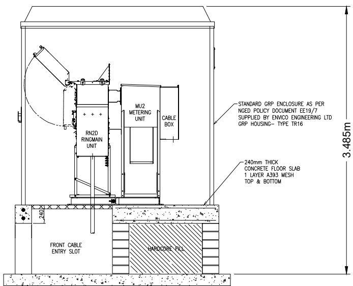
SECTION C-C
