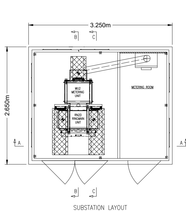
SUBSTATION LAYOUT
