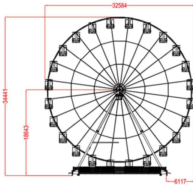
Front / rear elevation and dimensions
