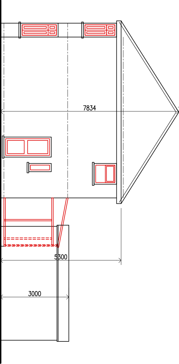
EXISTING DRIVE SIDE ELEVATION.
