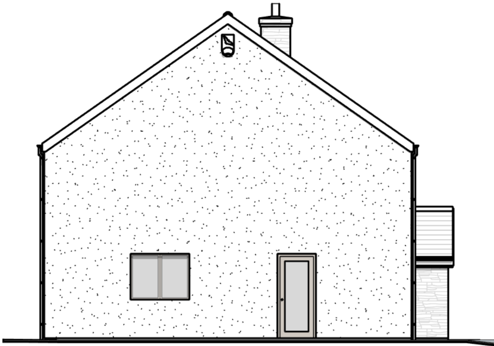
01 House Side Elevation (West) 1 : 100
