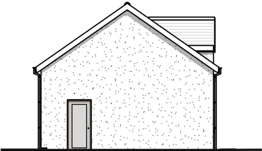
02 Garage Side Elevation (East) 1 : 100
