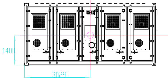
SIDE ELEVATION (TYPICAL FOR BOTH SIDES)
