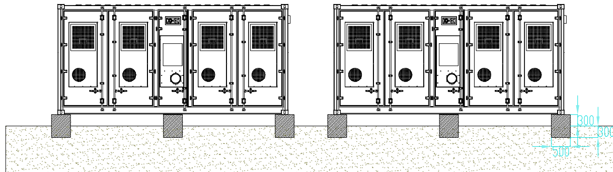
SIDE ELEVATION (TYPICAL FOR BOTH SIDES) - FOUNDATIONS
