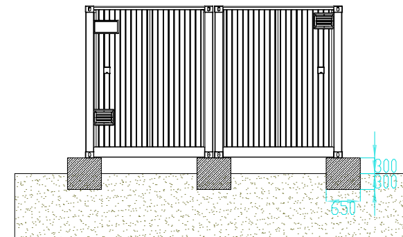
FRONT AND REAR ELEVATIONS - FOUNDATIONS
