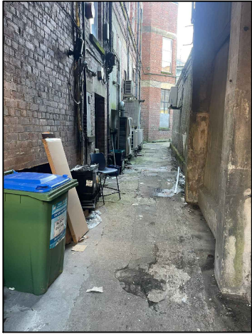
ELEVATION FROM SIDE LANE SHOWING LOCATION OF SHOOTERS AIR CON CONDENSERS
