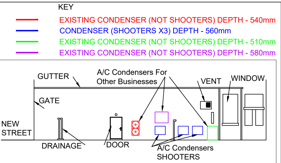
ELEVATION FROM SIDE LANE SHOWING LOCATION OF SHOOTERS AIR CON CONDENSERS
