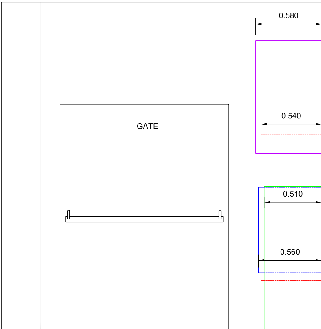
ELEVATION DOWN SIDE LANE FROM GATE ON NEW STREET
