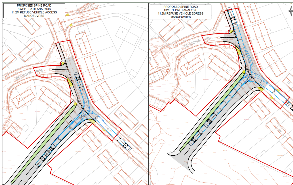
Figure 4.3 – Proposed Access Track Plots 11.2m Refuse Vehicle.
