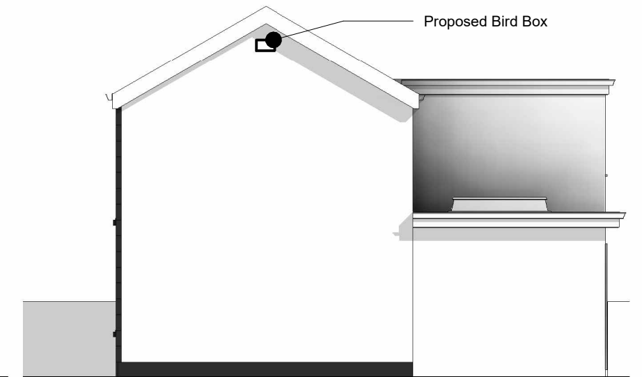
5 Proposed Side Elevation (2) 1 : 100
