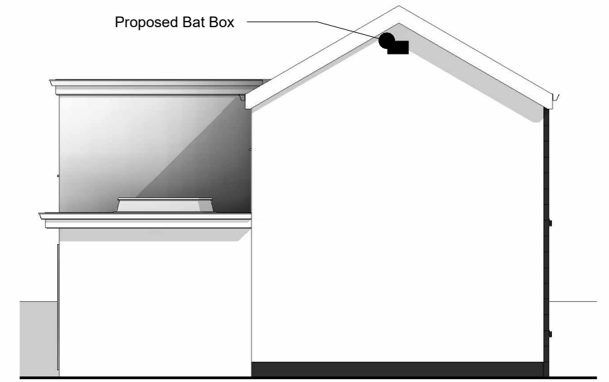
4 Proposed Side Elevation (1) 1 : 100
