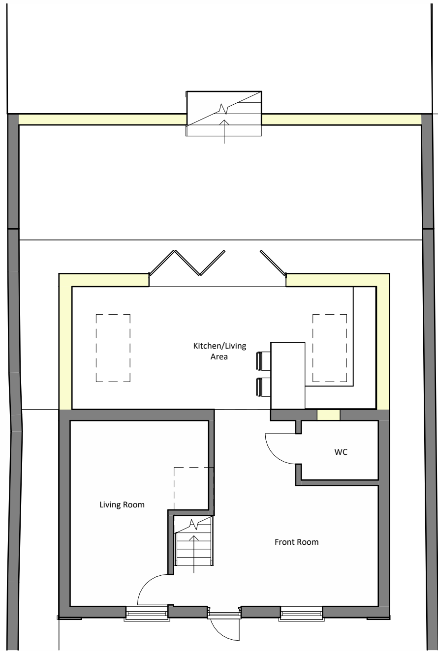
1 1.2 - Proposed Ground Floor 1 : 100
