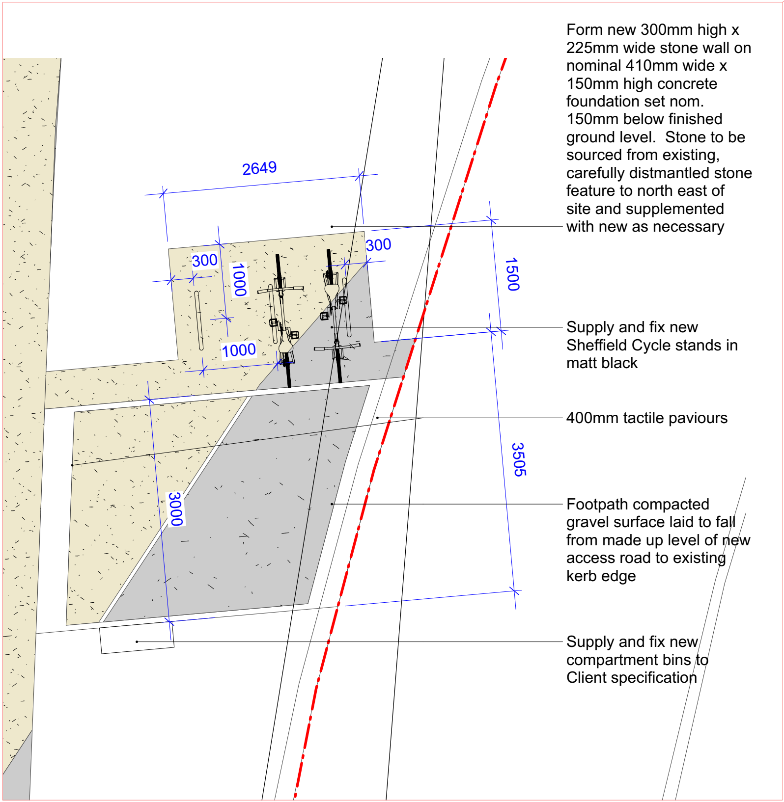
01320.02 PARKING LAYOUT SCALE 1:50 @ A1, 1:100 @ A3
