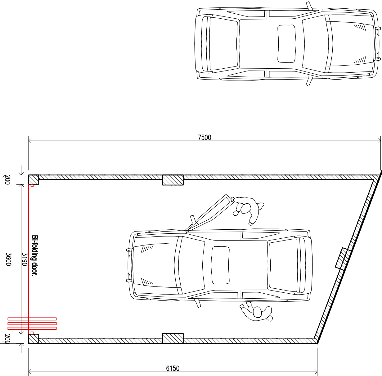
PROPOSED GROUND FLOOR PLAN. (1:50)
