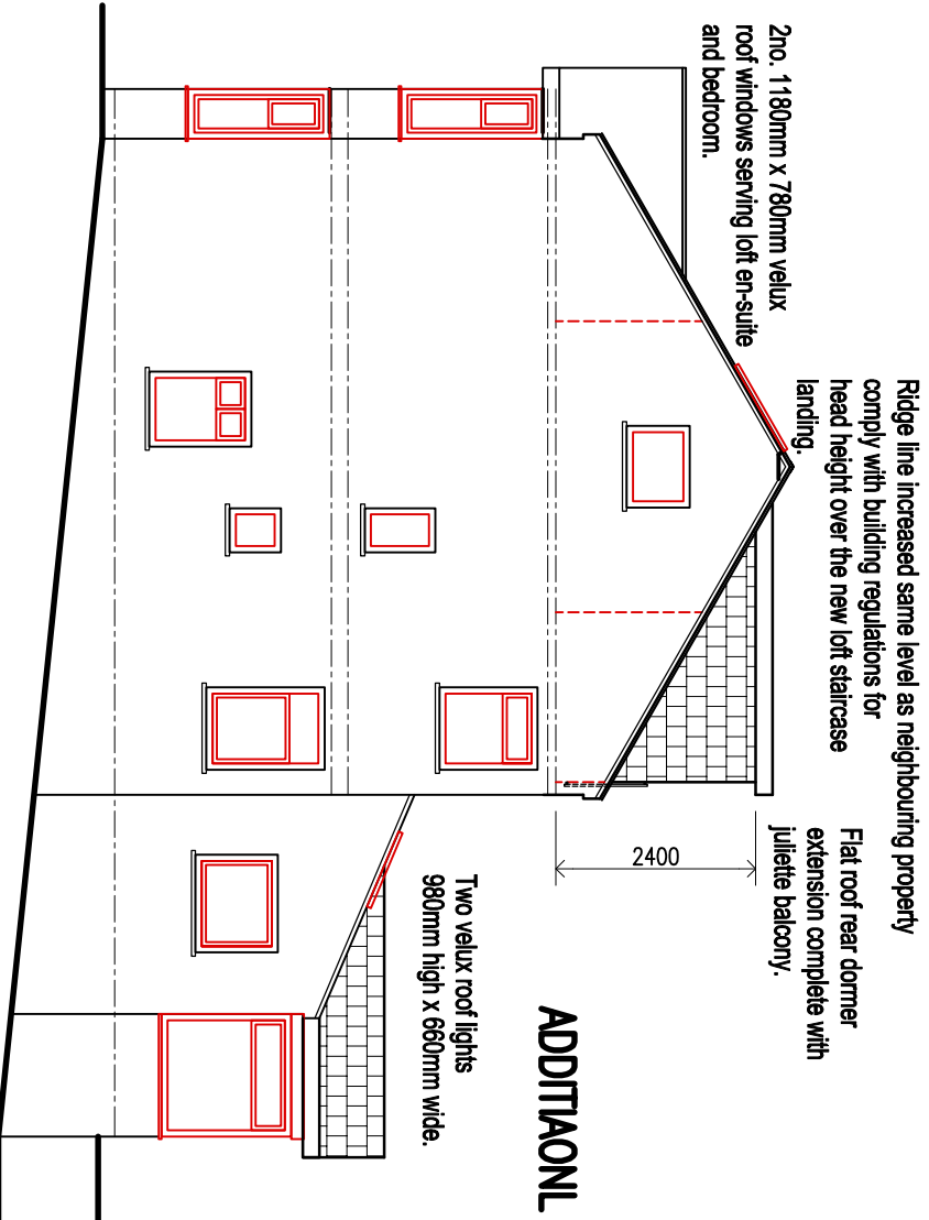
PROPOSED SIDE ELEVATION. (1:100)
