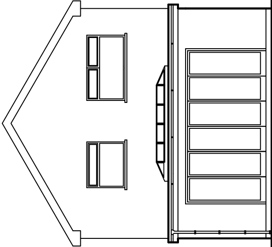
REAR ELEVATION
