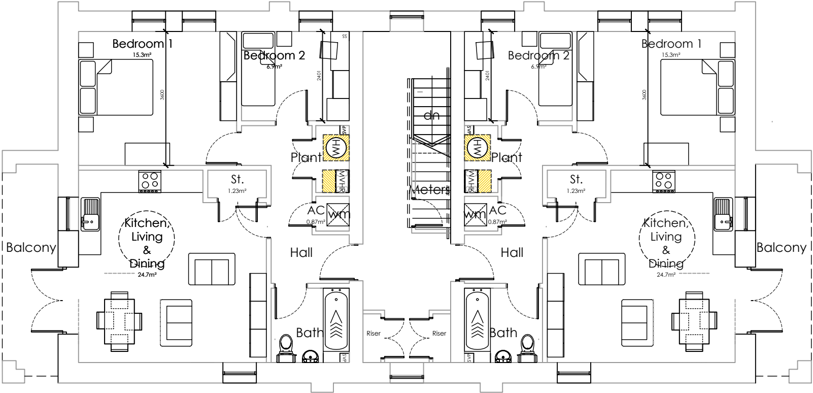
BUILDING TYPE A: FIRST FLOOR PLAN
