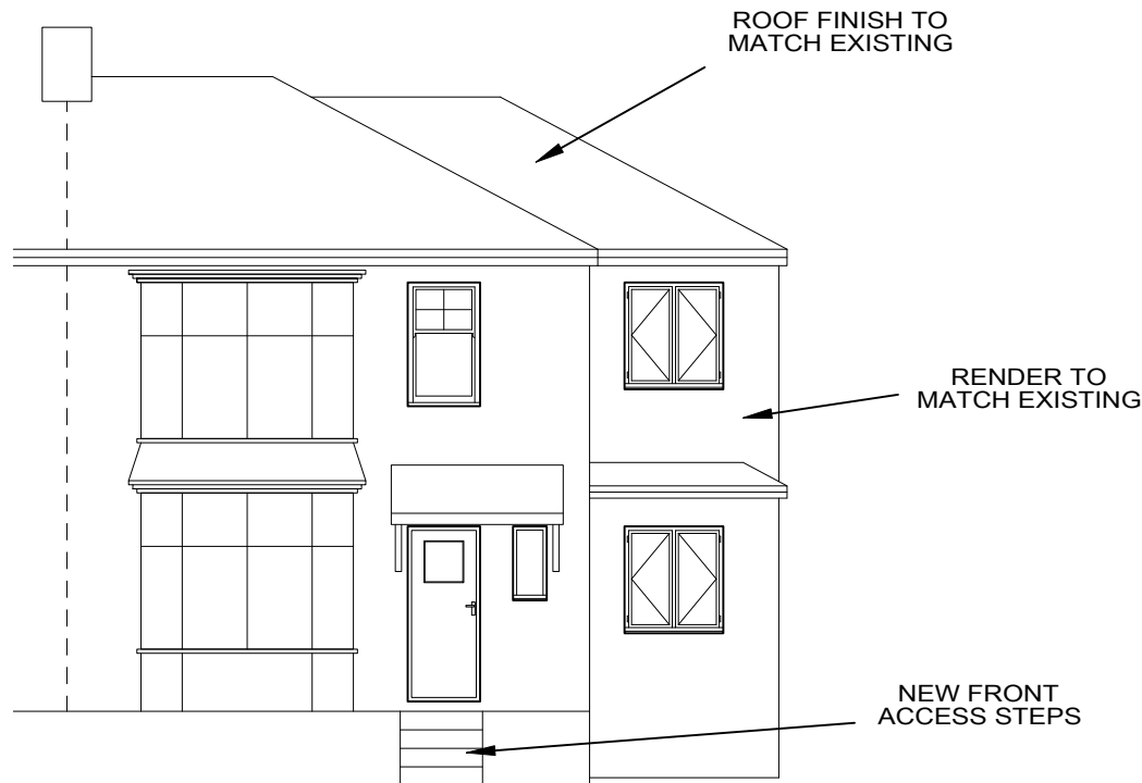
FRONT ELEVATION PROPOSED
