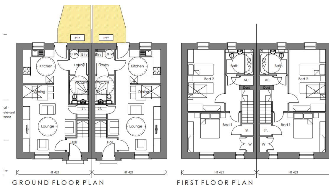
Figure 5: Excerpt from 2617-421(03)200 - Plans & Elevations 421
