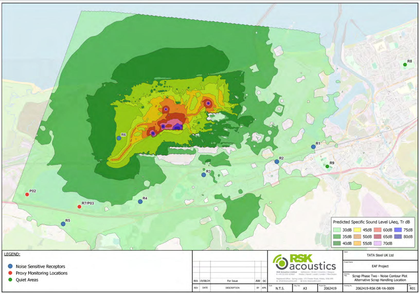
Figure C 10 Noise Contour Plot – Phase Two (Alternative scrap handling location)
