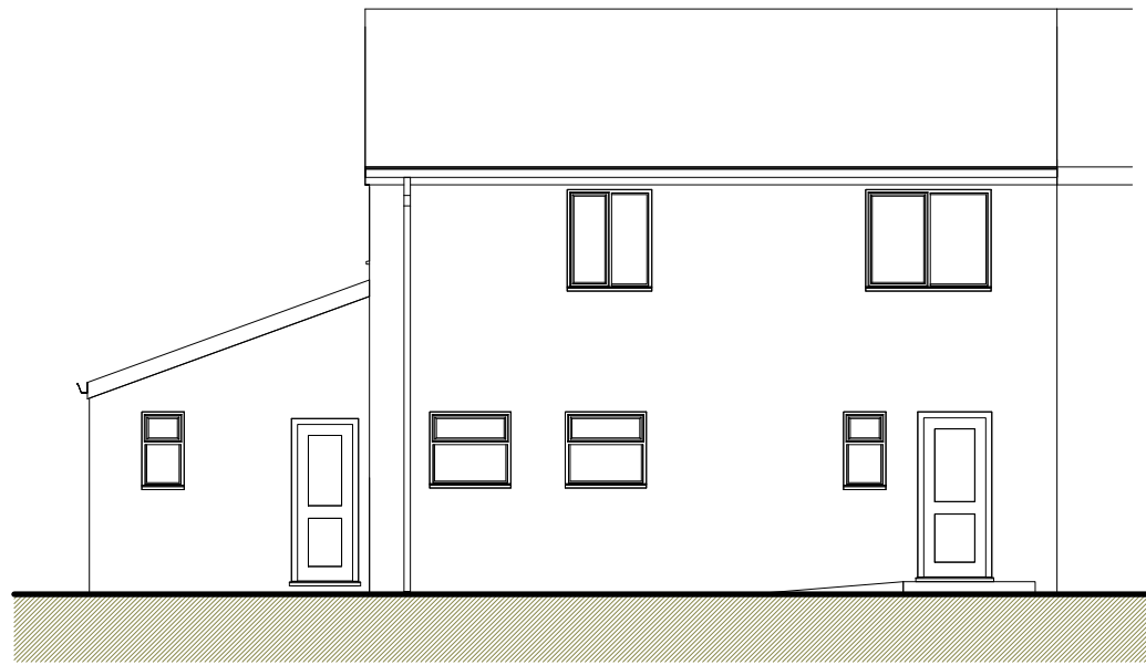
1 Front elevation 1 : 100
