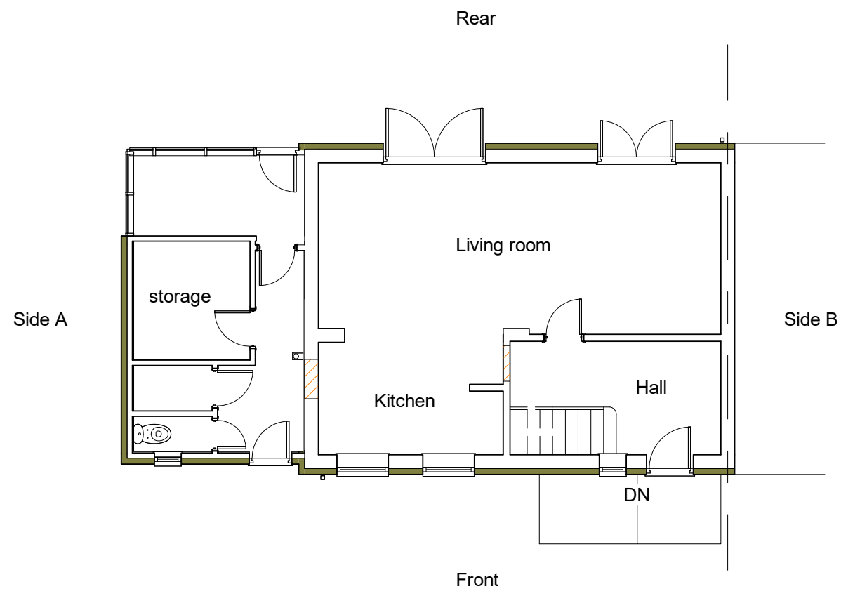
1 ground floor 1 : 100
