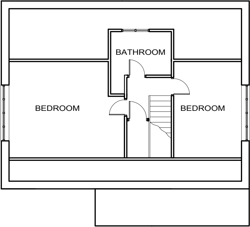
FIRST FLOOR PLAN EXISTING
