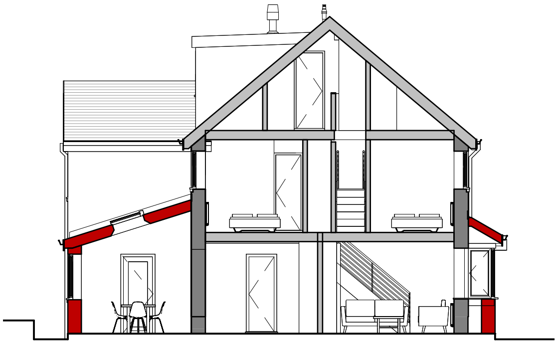
Proposed Section
