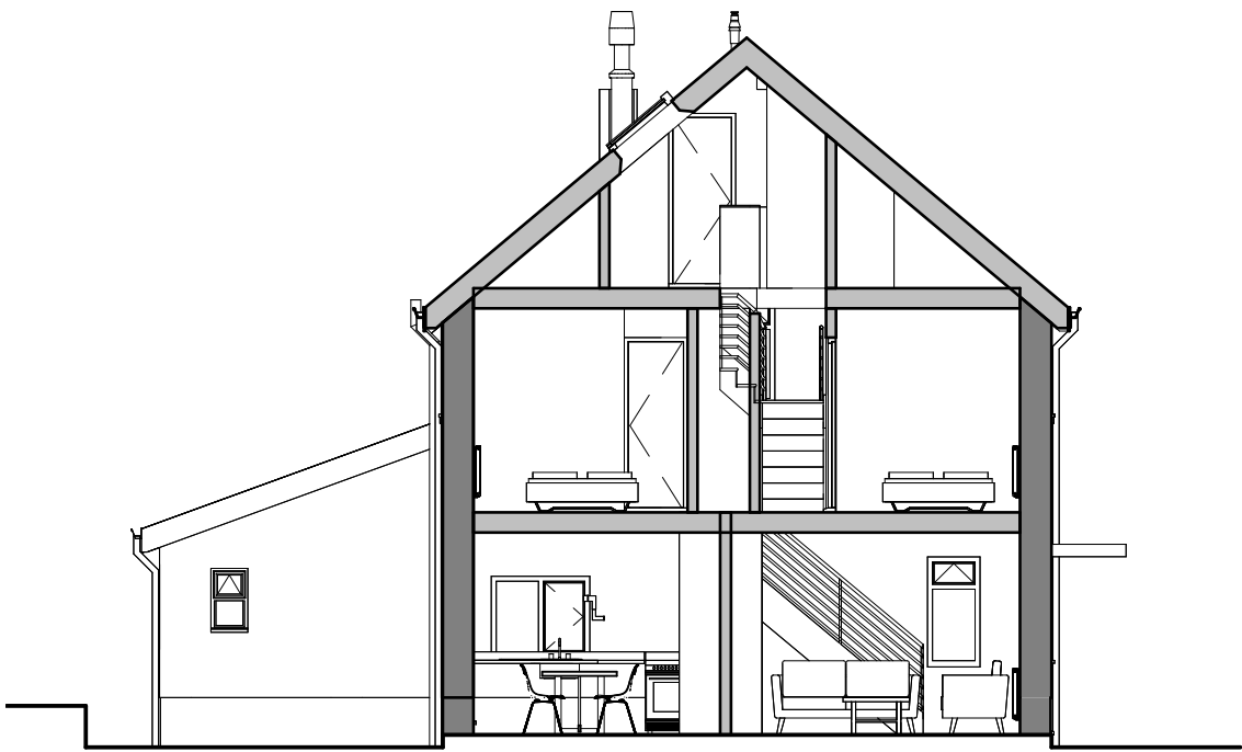
Existing Section
