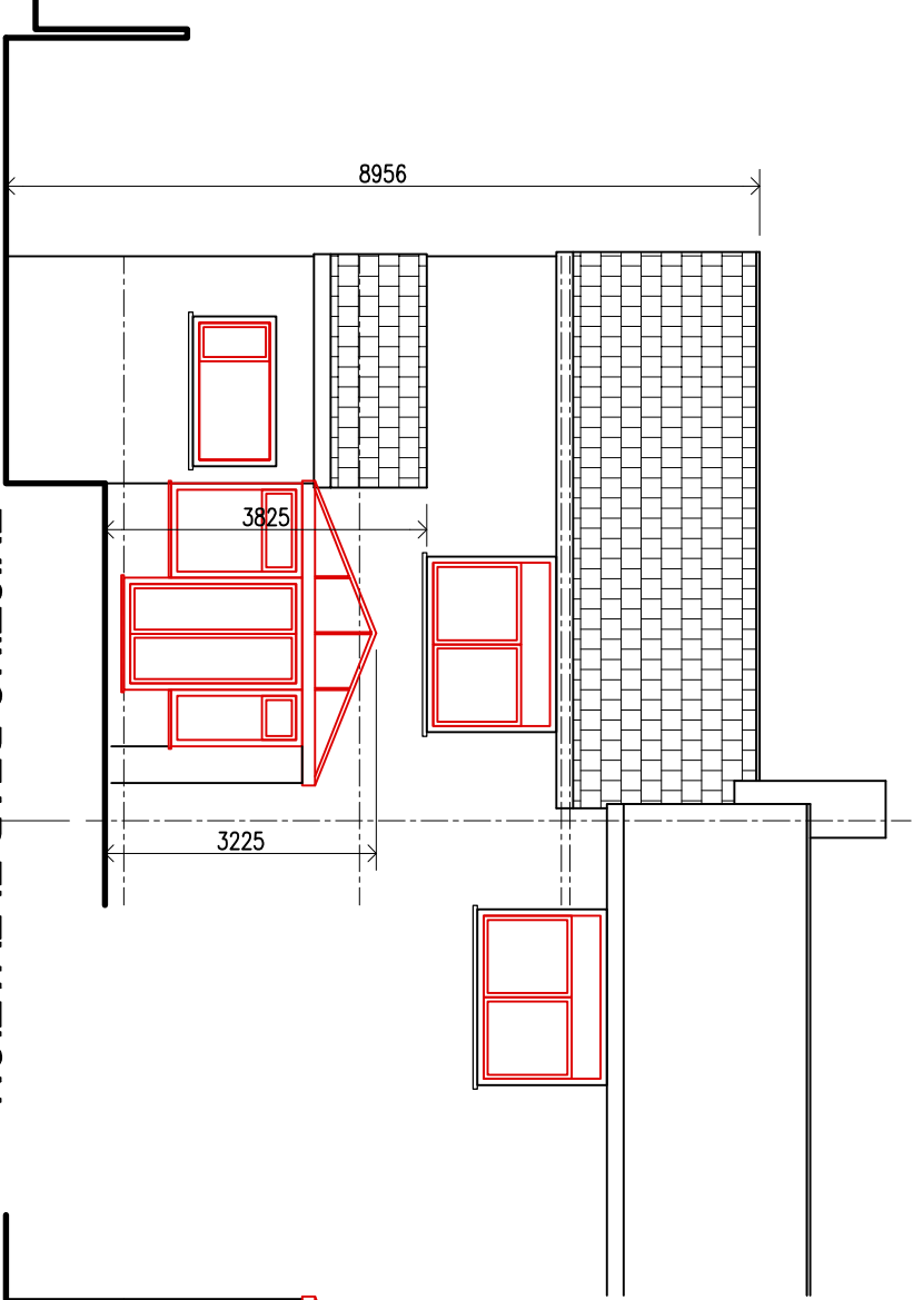
EXISTING REAR ELEVATION. (1:100)
