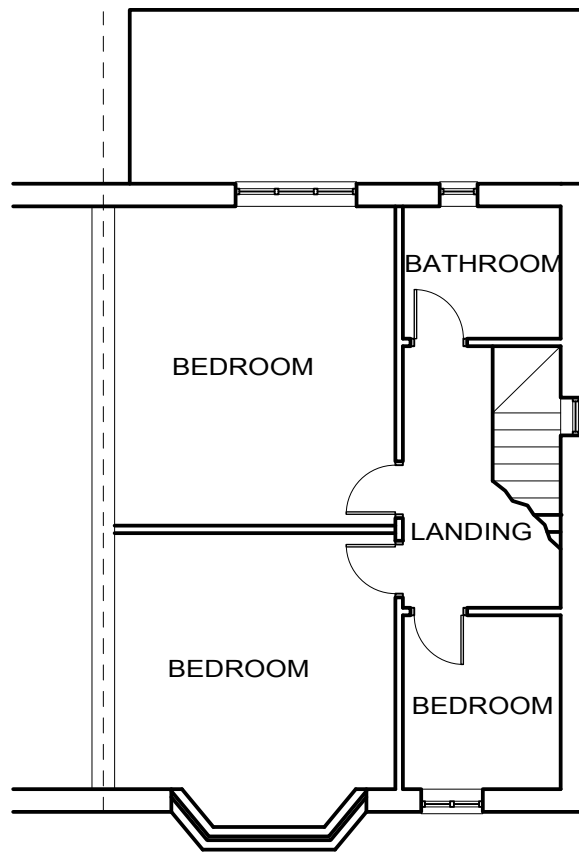
FIRST FLOOR PLAN EXISTING
