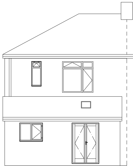
REAR ELEVATION EXISTING
