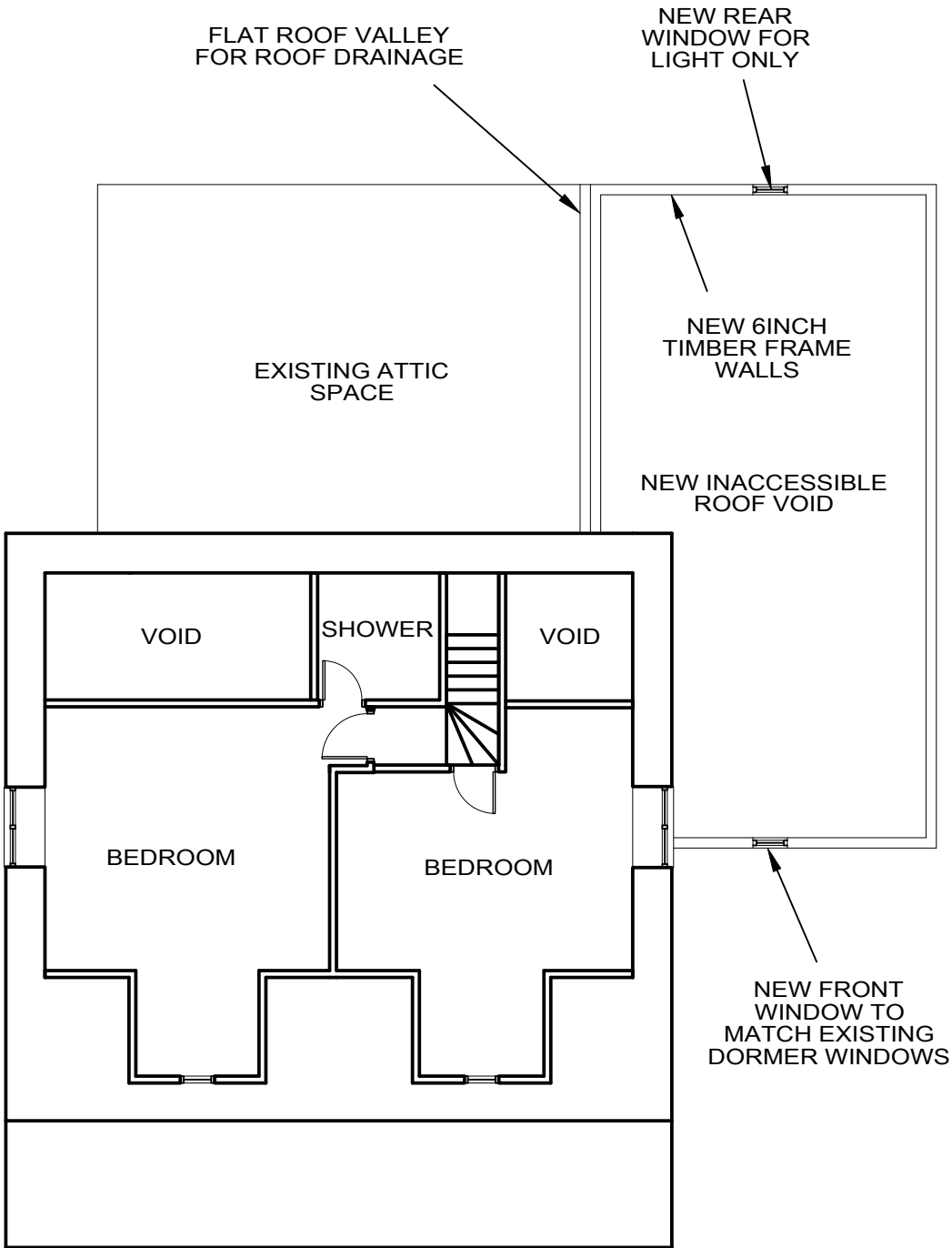
SECOND FLOOR PLAN PROPOSED
