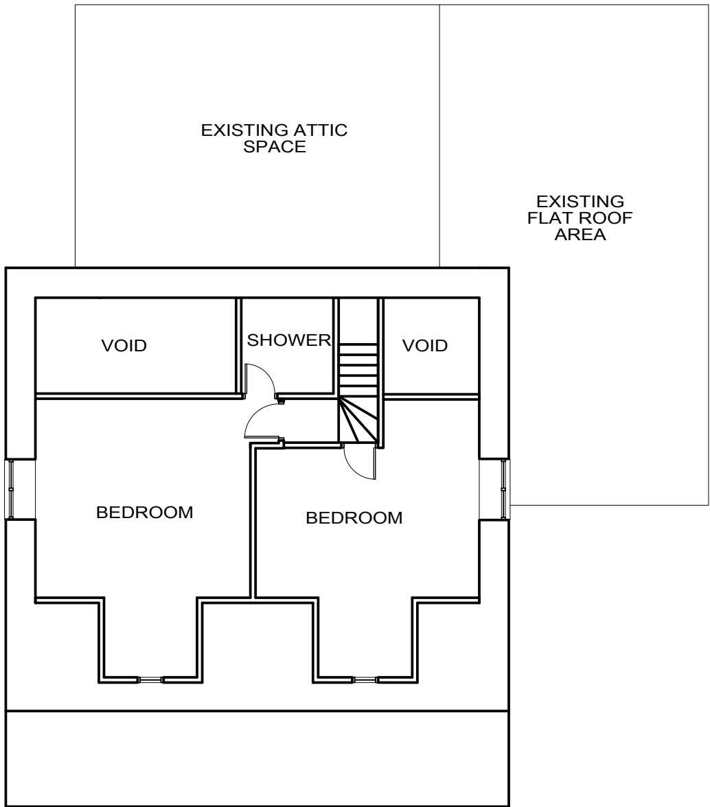
SECOND FLOOR PLAN EXISTING
