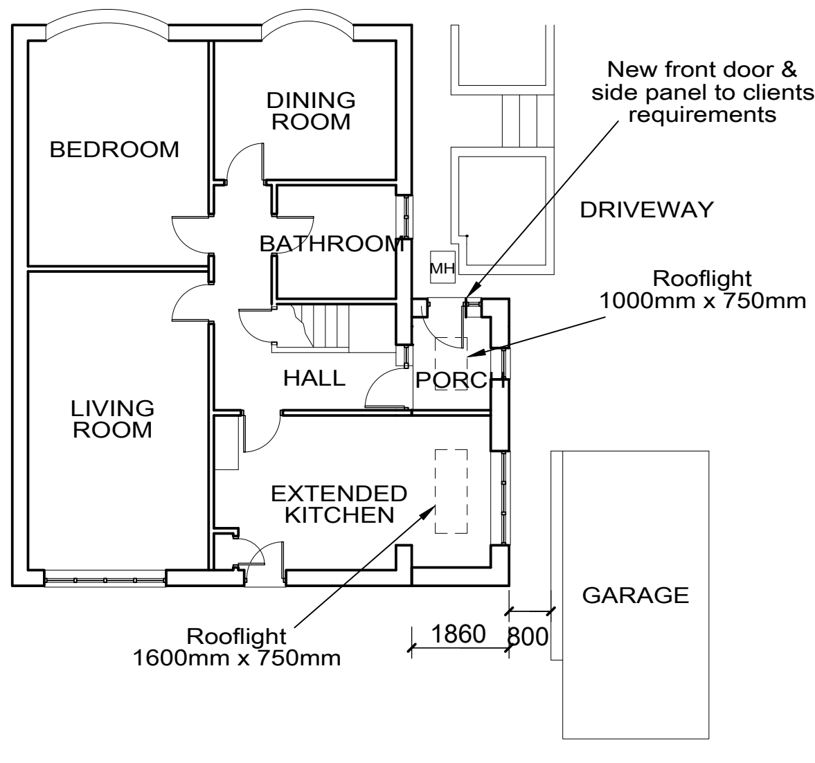
GROUND FLOOR PLAN PROPOSED
