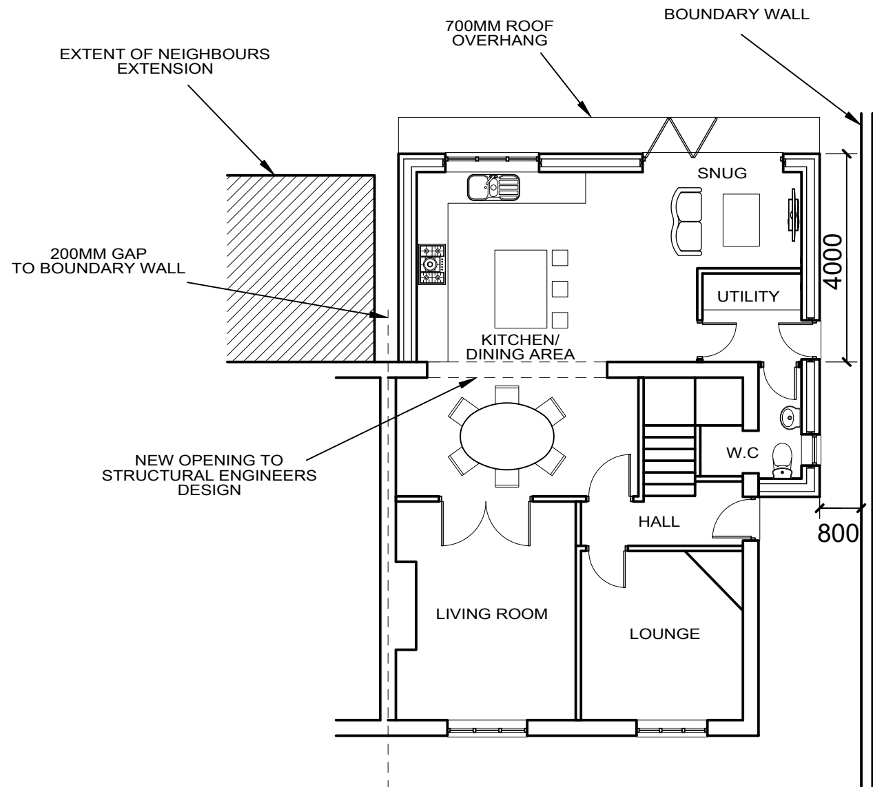
GROUND FLOOR PLANS PROPOSED
