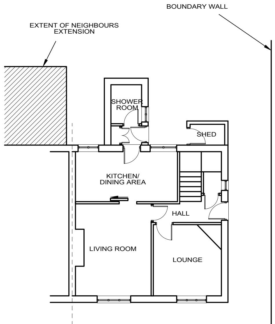
GROUND FLOOR PLANS EXISTING
