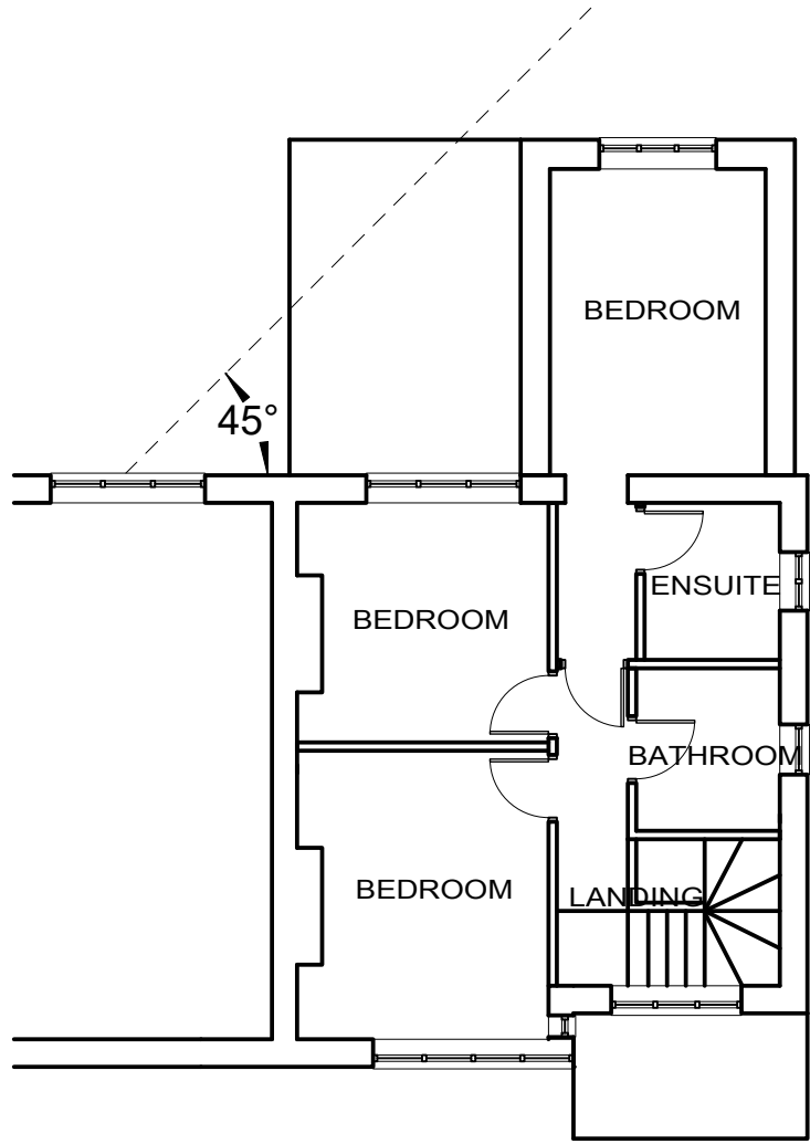
FIRST FLOOR PLAN PROPOSED
