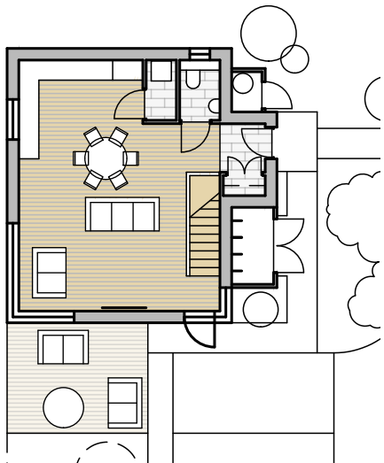
lodge type A: 2 bed split level
