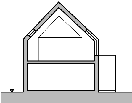
section for room in roof house types D and E
