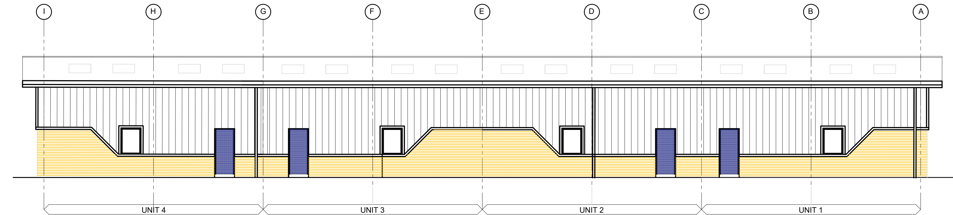
REAR ELEVATION
