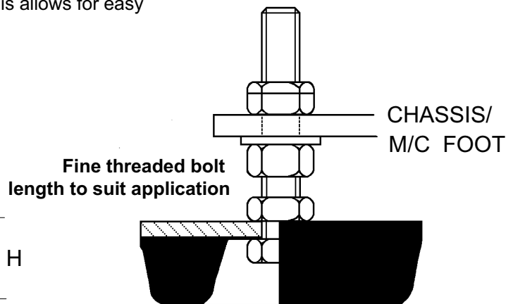
HEIGHT ADJUSTMENT ARRANGEMENT (NOT SUPPLIED)
