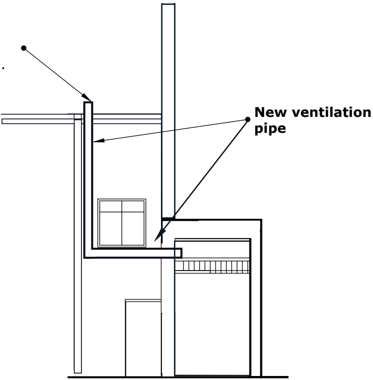
SIDE (SOUTH-EAST) ELEVATION - PROPOSED
