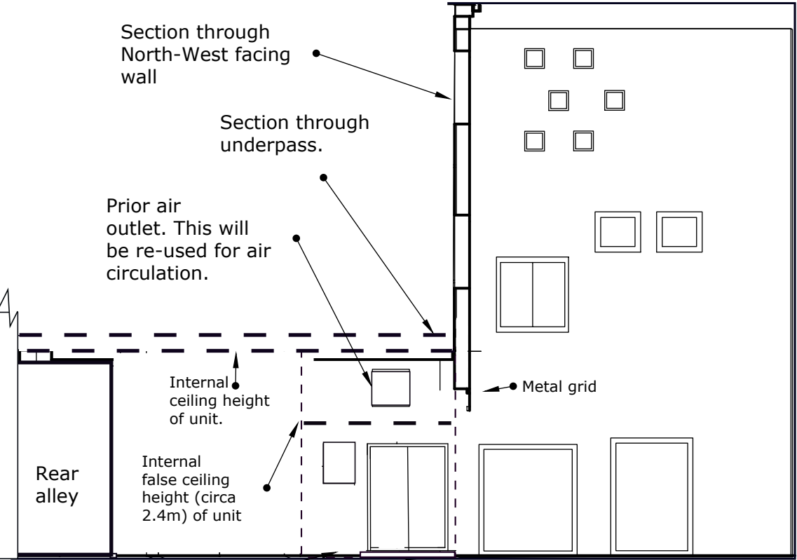
REAR (NORTH-EAST) ELEVATION - EXISTING
