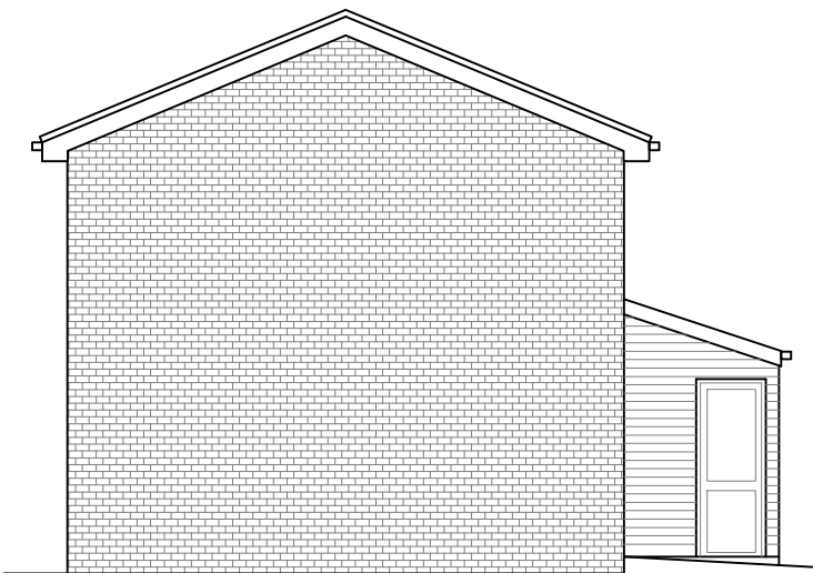
ELEVATION TO NORTH/WEST
