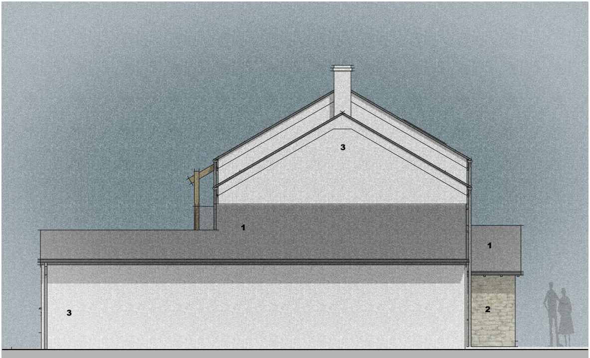
SIDE ELEVATION
