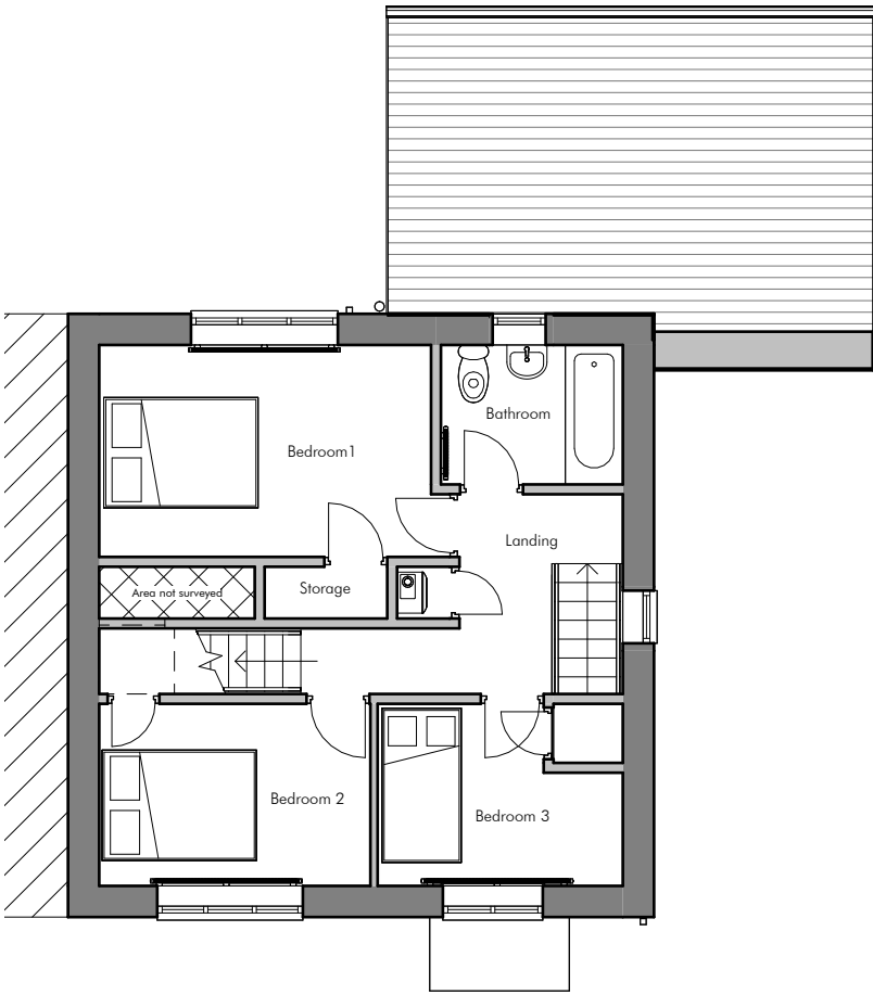
First Floor
