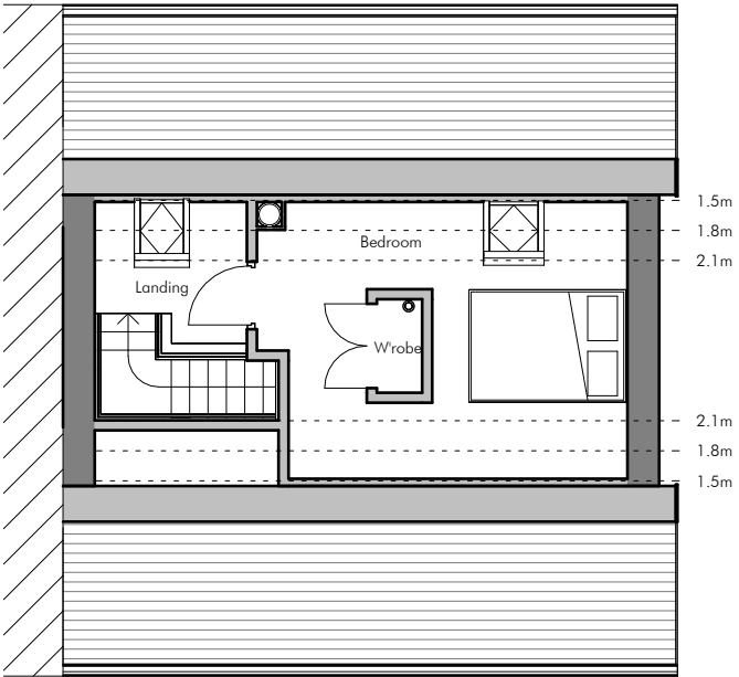
Attic Floor
