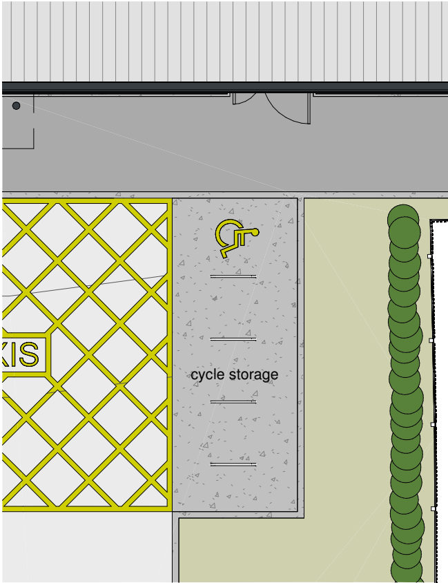
Cycle Store Key 1 : 100
