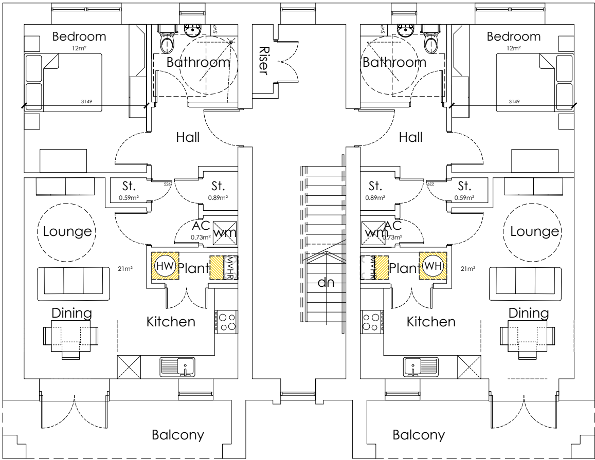
BUILDING TYPE D: SECOND FLOOR PLAN
