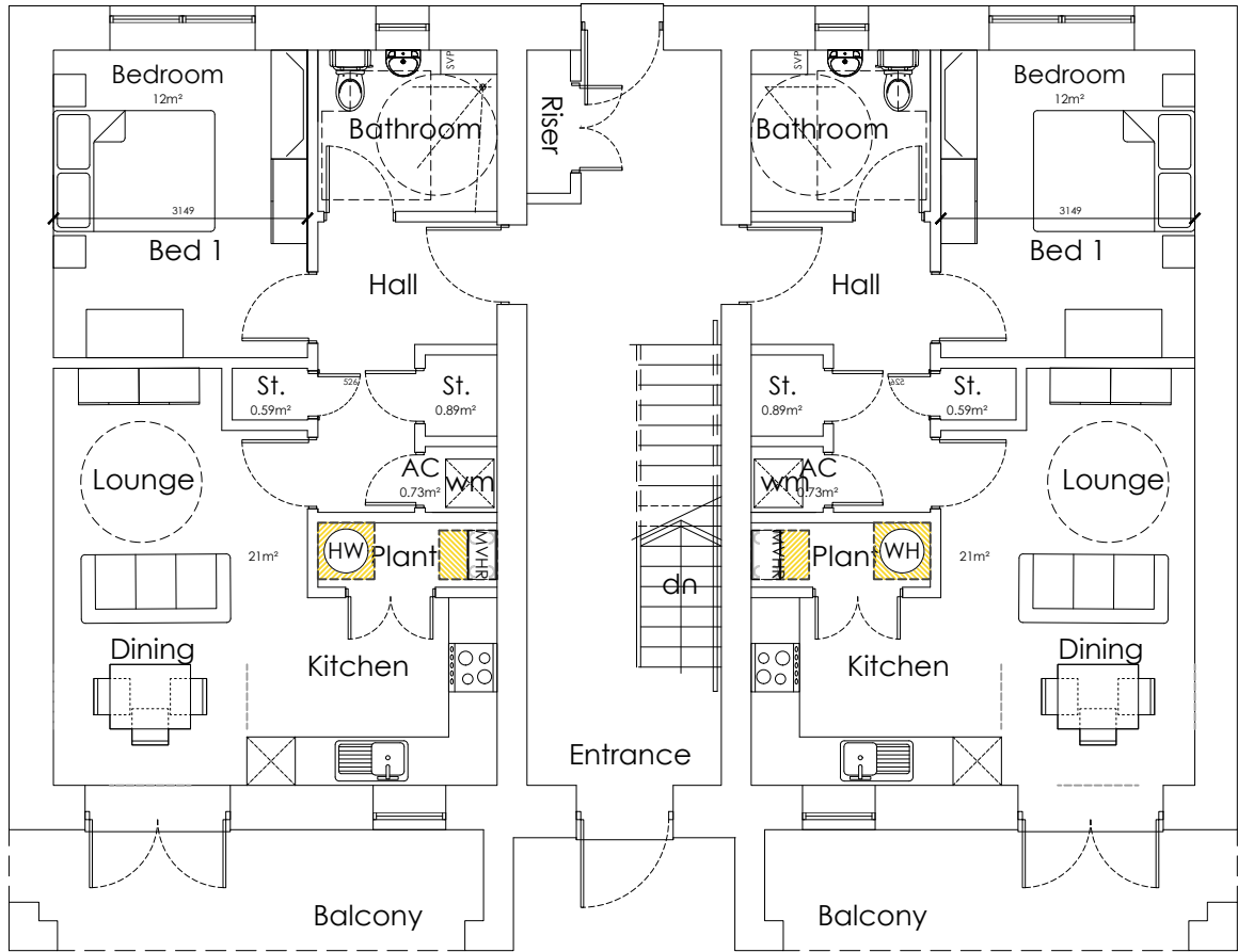
BUILDING TYPE D: GROUND FLOOR PLAN
