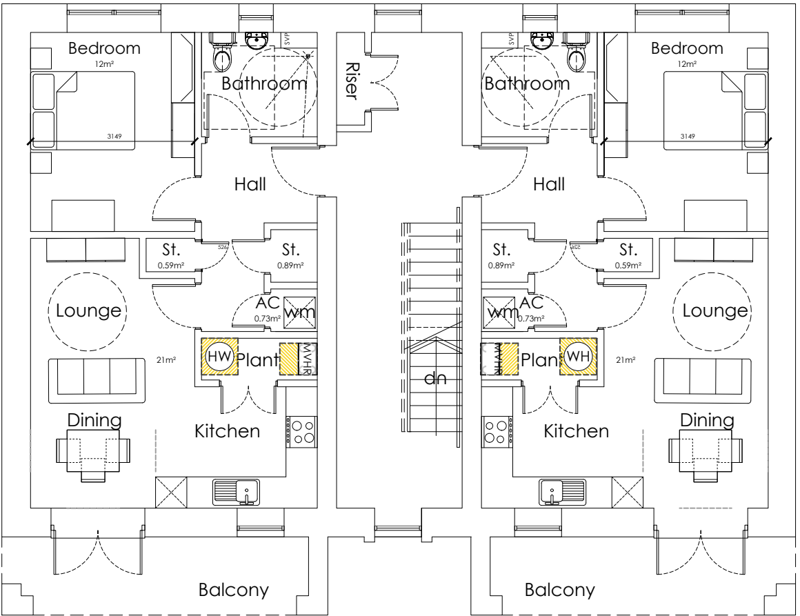
BUILDING TYPE D: FIRST FLOOR PLAN
