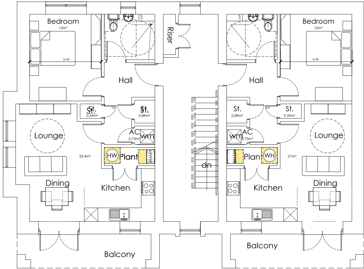
BUILDING TYPE B: SECOND FLOOR PLAN
