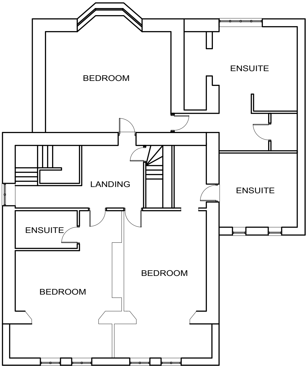
FIRST FLOOR PLAN EXISTING & PROPOSED (NO ALTERATIONS AS ROOF IS PURELY FOR AESTHETIC & MAINTENANCE PURPOSES & IS NOT ACCESSIBLE AS A ROOM)
