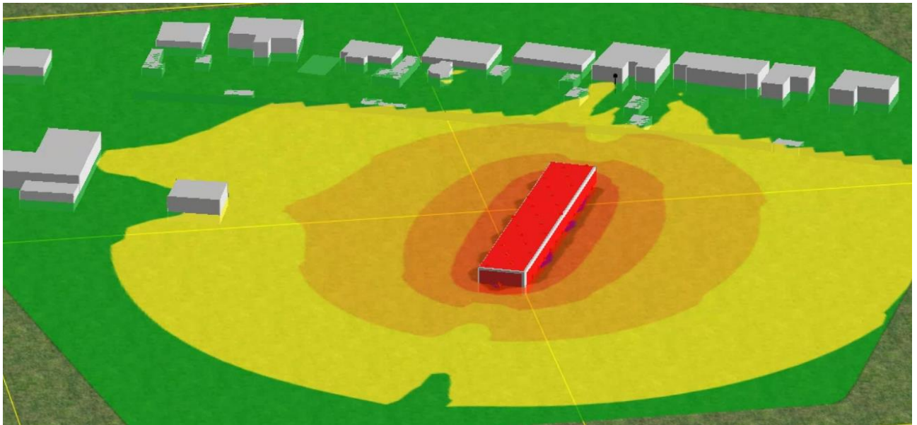
FIGURE 7: 3D VIEW OF NOISE PROPAGATION FOR LOUDEST SINGLE ITEM (LOOKING DUE WEST) AT 2M HEIGHT (ROLLER SHUTTERS CLOSED)
