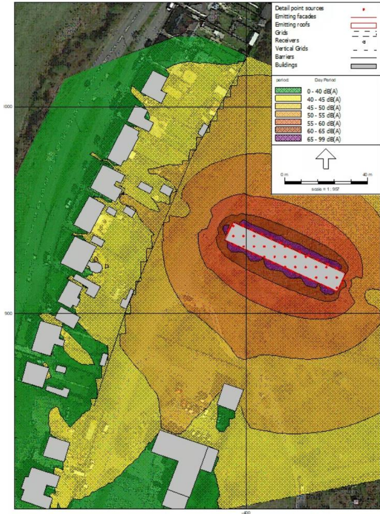
FIGURE 8: NOISE CONTOURS ACROSS THE SITE FOR TOTAL 2 SCENARIO AT 2M HEIGHT (ROLLER SHUTTERS CLOSED)
