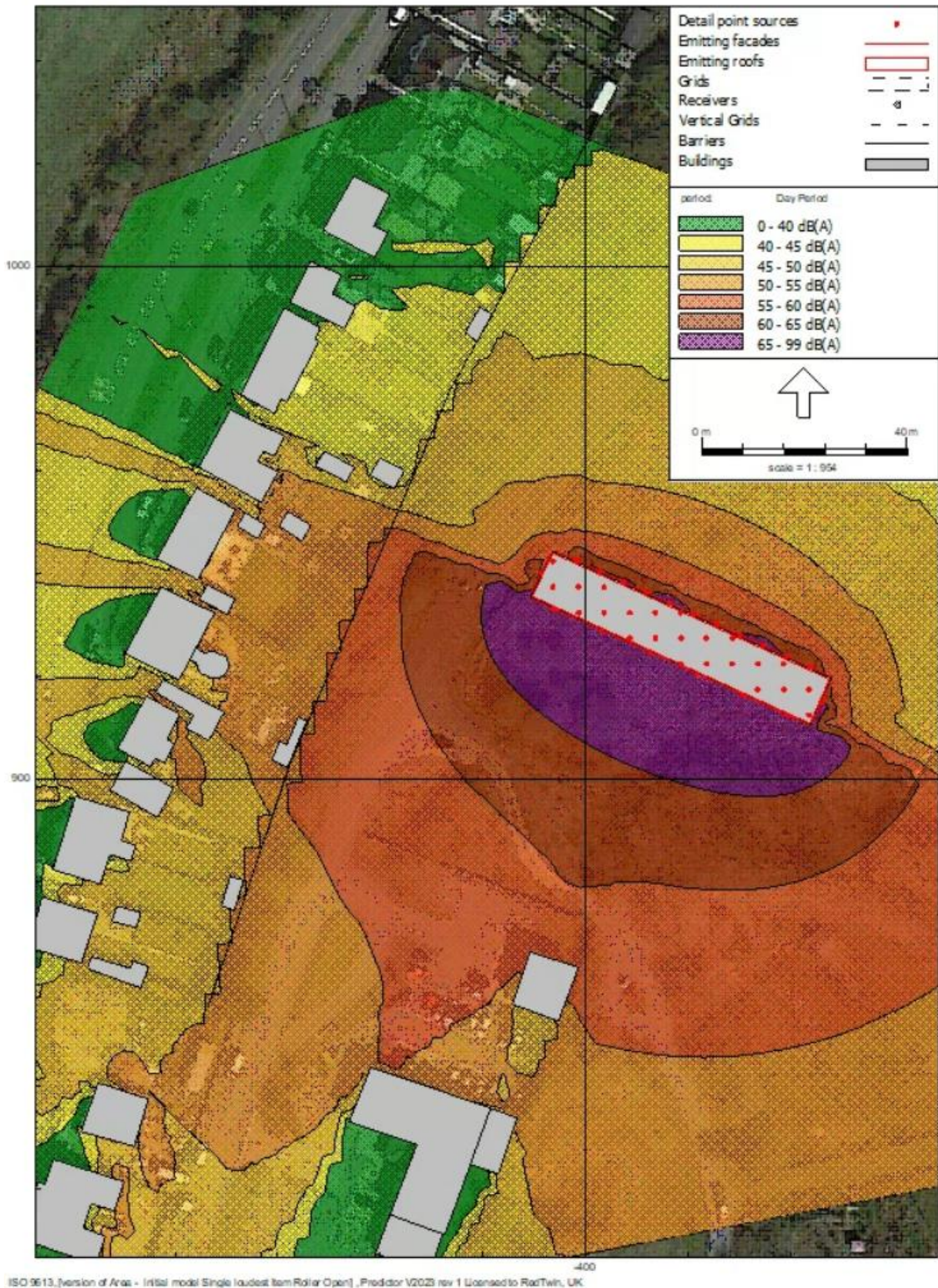
FIGURE 6: NOISE CONTOURS ACROSS THE SITE FOR LOUDEST SINGLE ITEM AT 2M HEIGHT (ROLLER SHUTTERS OPEN)
