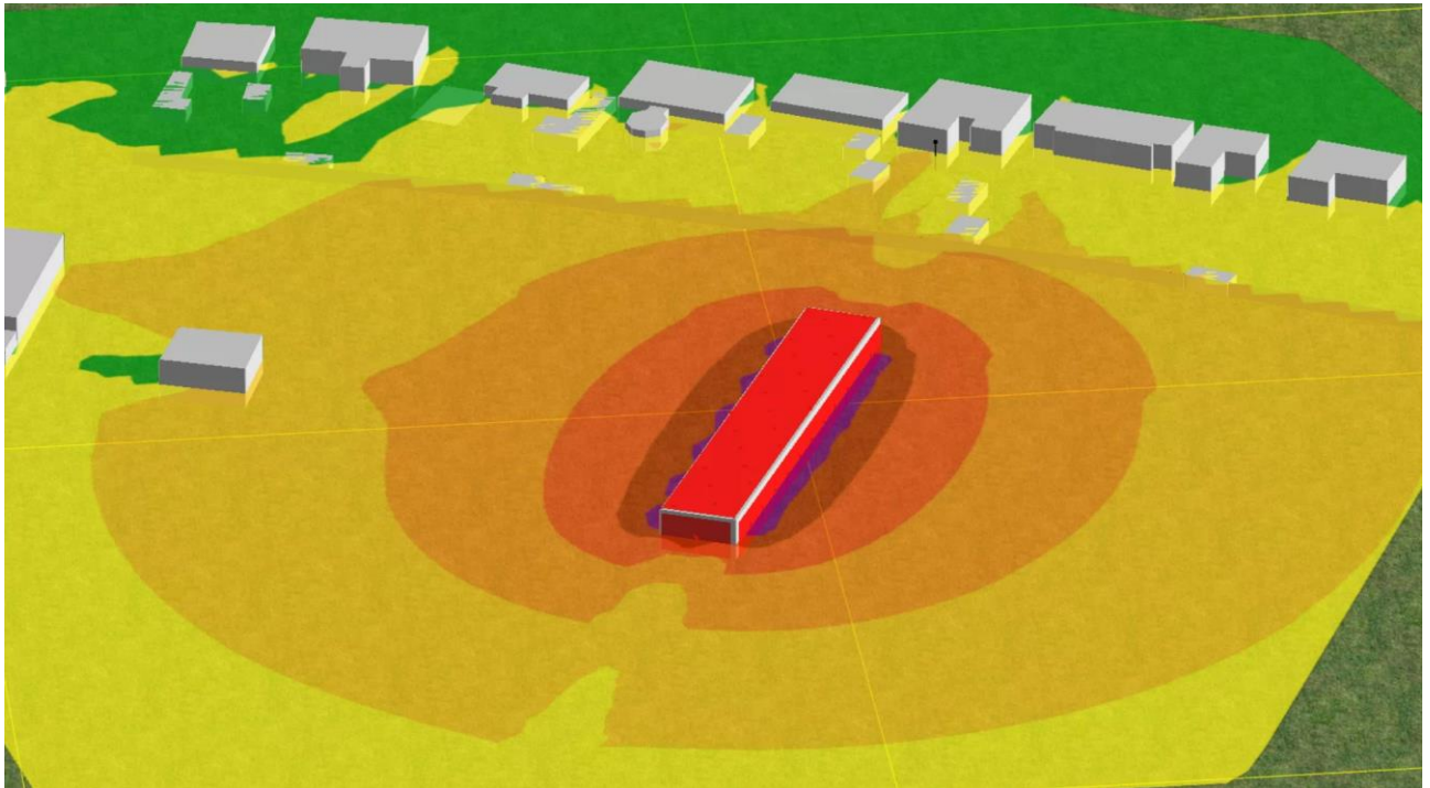
FIGURE 10: 3D VIEW OF NOISE PROPAGATION FOR TOTAL 2 SCENARIO (LOOKING DUE WEST) AT 2M HEIGHT (ROLLER SHUTTERS CLOSED)
