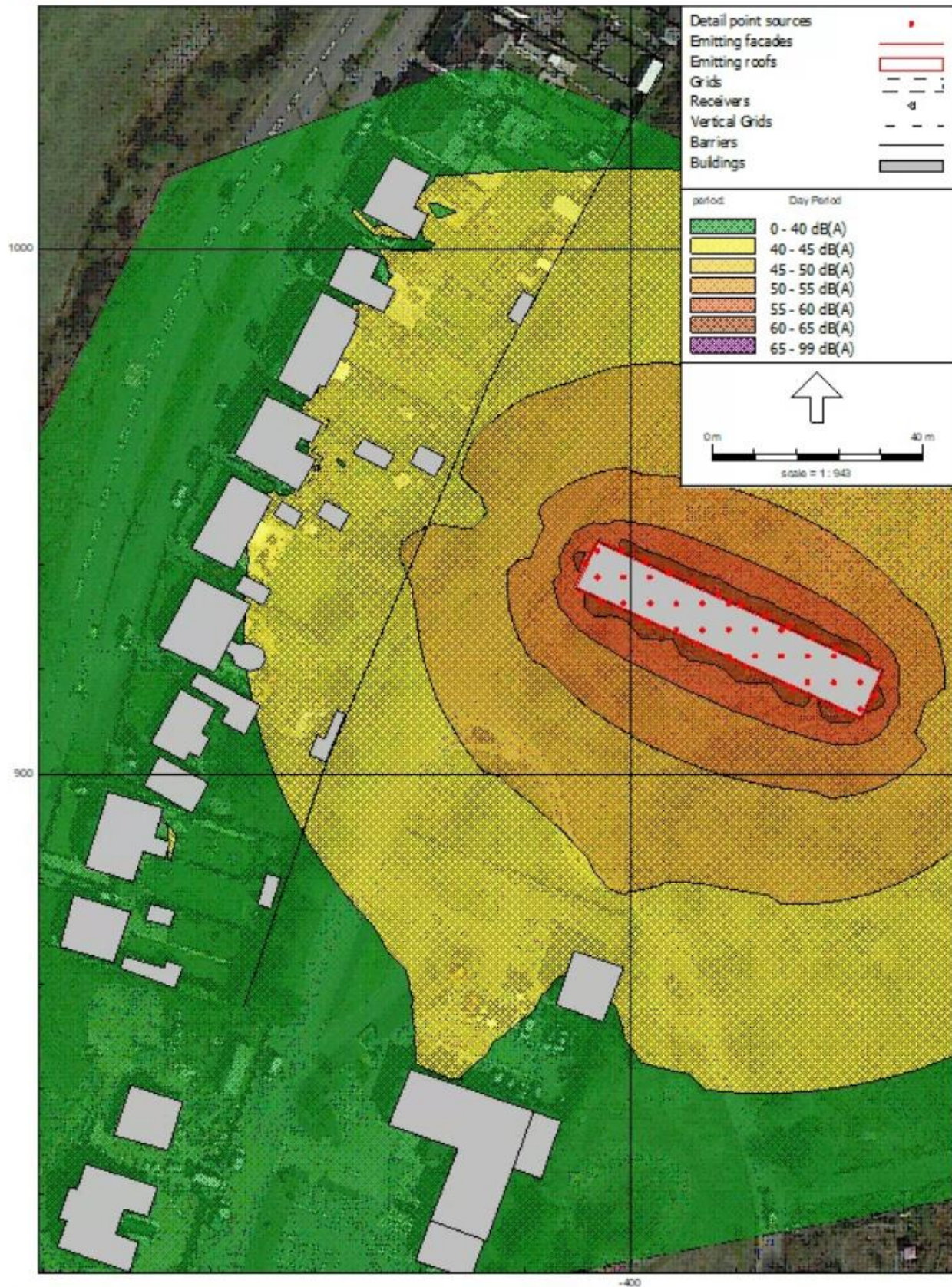
FIGURE 5: NOISE CONTOURS ACROSS THE SITE FOR LOUDEST SINGLE ITEM AT 2M HEIGHT (ROLLER SHUTTERS CLOSED)
