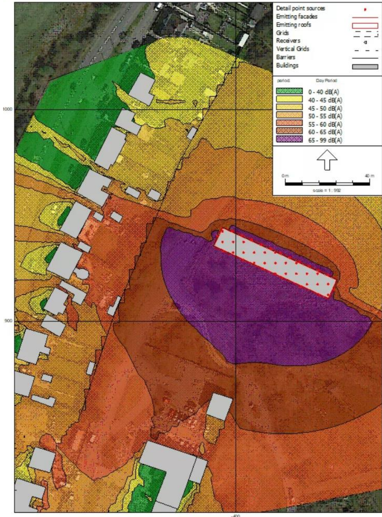
FIGURE 9: NOISE CONTOURS ACROSS THE SITE FOR TOTAL 2 SCENARIO AT 2M HEIGHT (ROLLER SHUTTERS OPEN)
