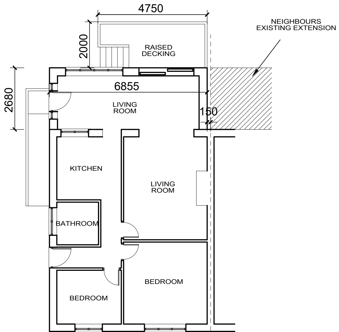
GROUND FLOOR PLAN PROPOSED
