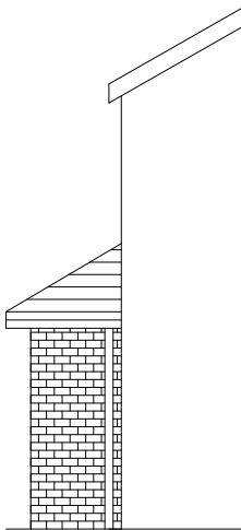
SIDE ELEVATION TO NEIGHBOUR EXISTING
